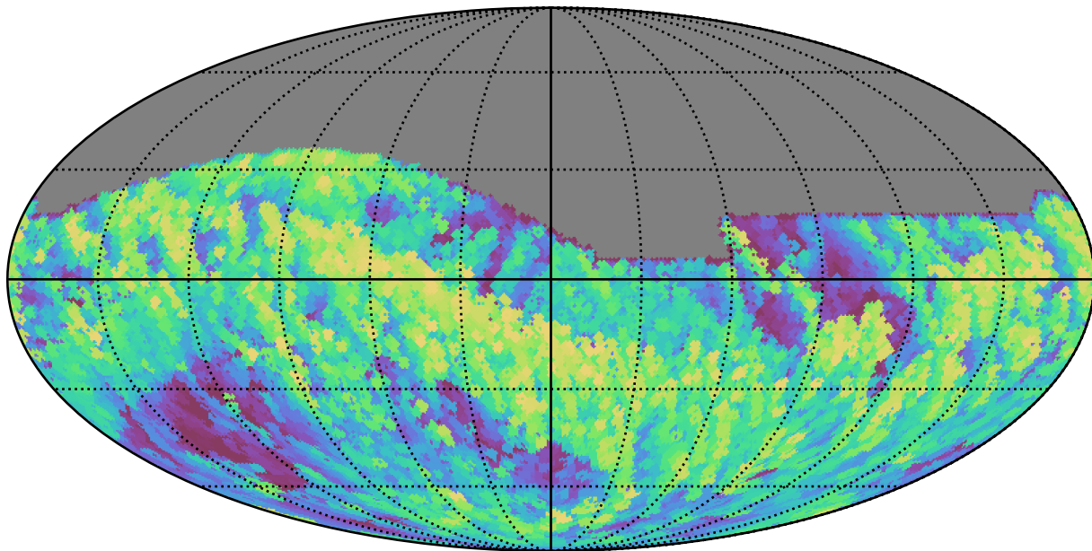
baseline_v3.5_10yrs All sky z band: Max airmass
