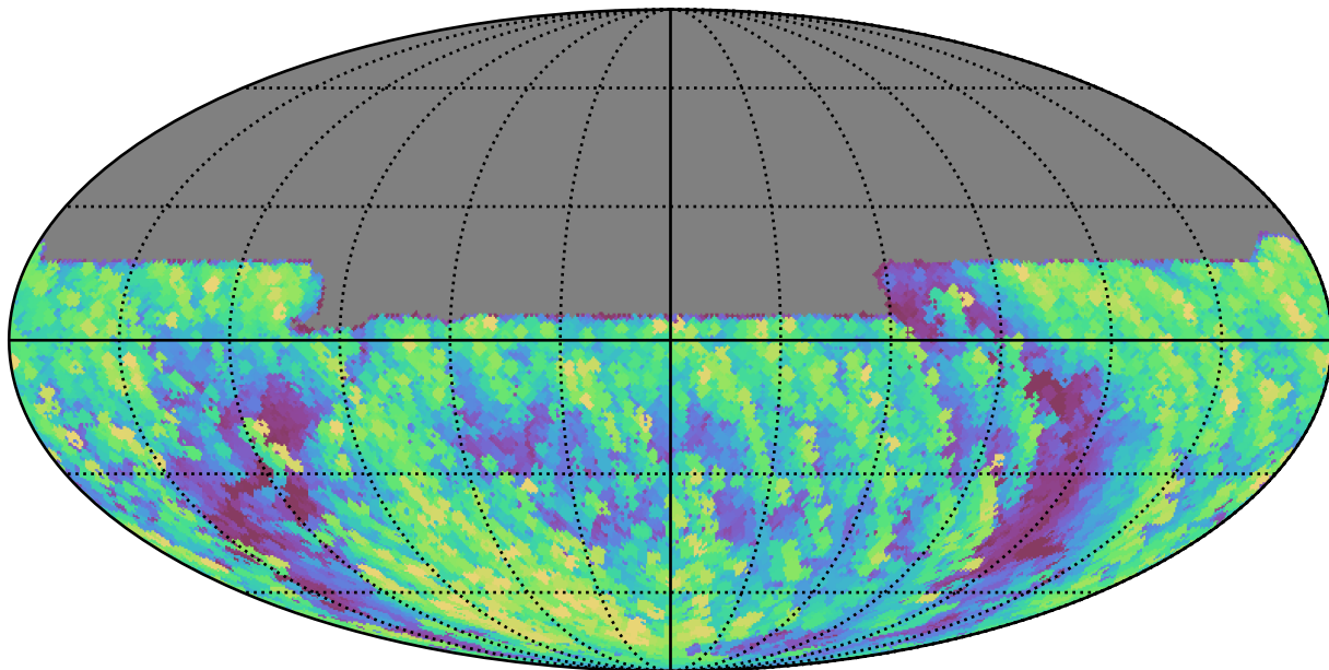
baseline_v3.5_10yrs All sky y band: Max airmass
