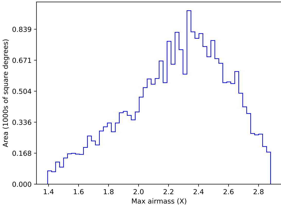
baseline_v3.5_10yrs All sky y band: Max airmass
