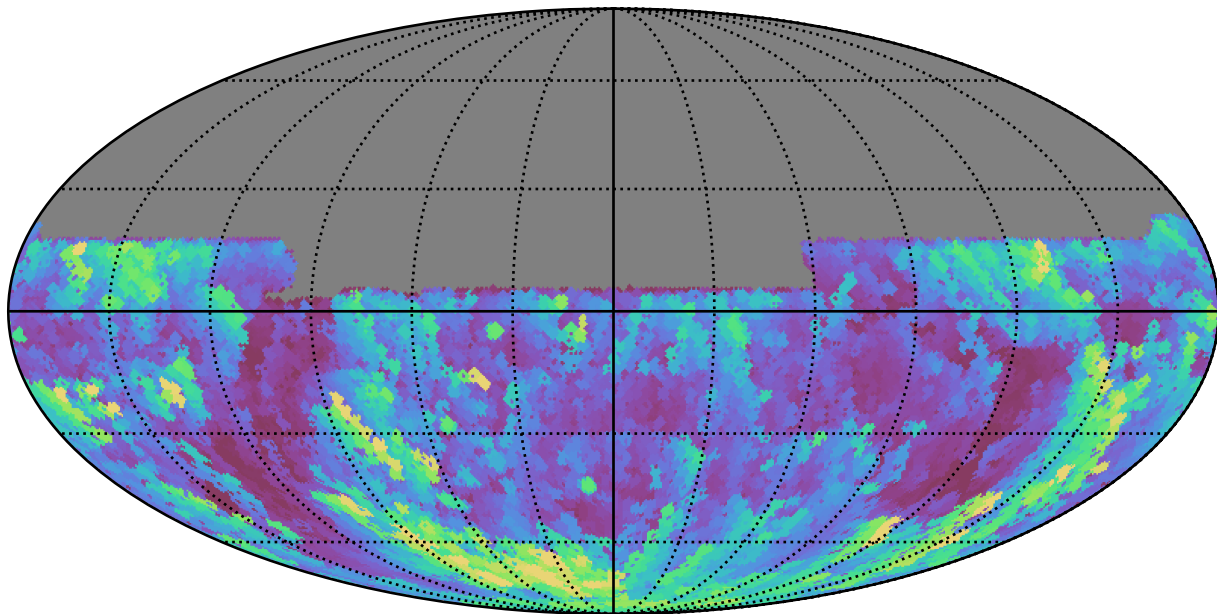
baseline_v3.5_10yrs All sky u band: Max airmass
