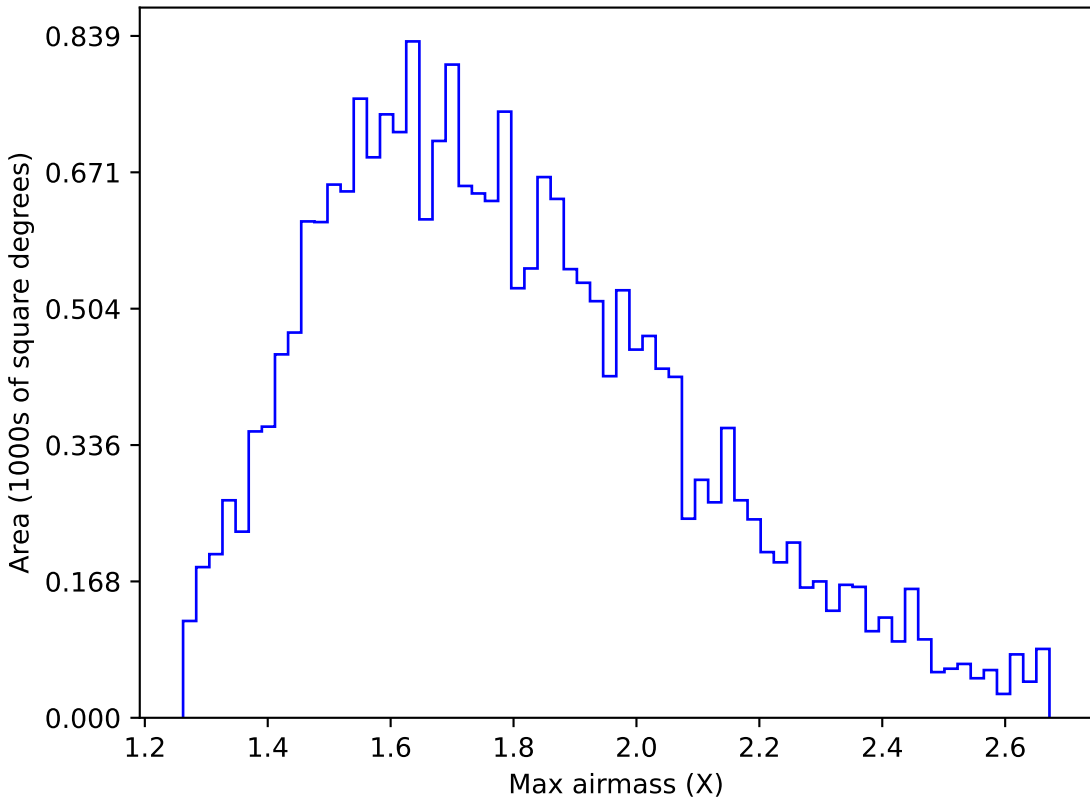
baseline_v3.5_10yrs All sky u band: Max airmass
