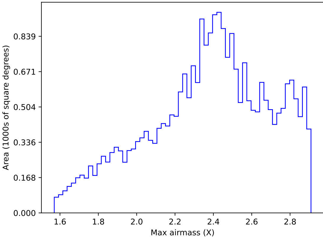
baseline_v3.5_10yrs All sky r band: Max airmass
