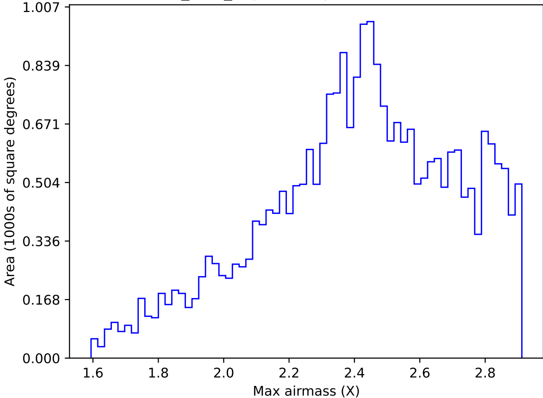
baseline_v3.5_10yrs All sky i band: Max airmass
