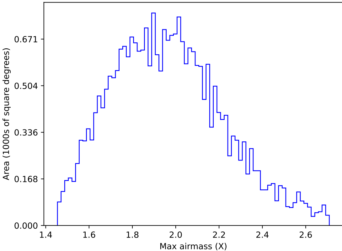
baseline_v3.5_10yrs All sky g band: Max airmass
