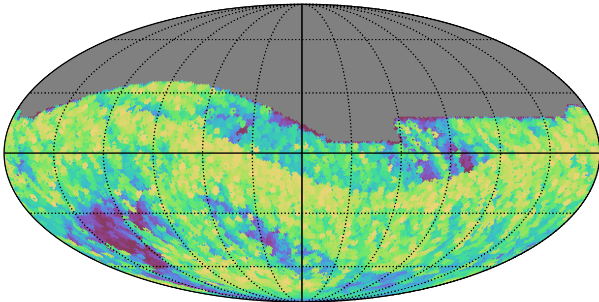
baseline_v3.5_10yrs All sky all bands: Max airmass
