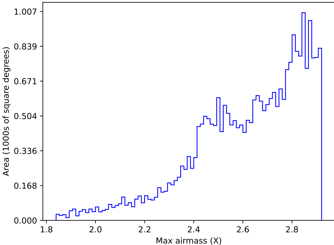
baseline_v3.5_10yrs All sky all bands: Max airmass
