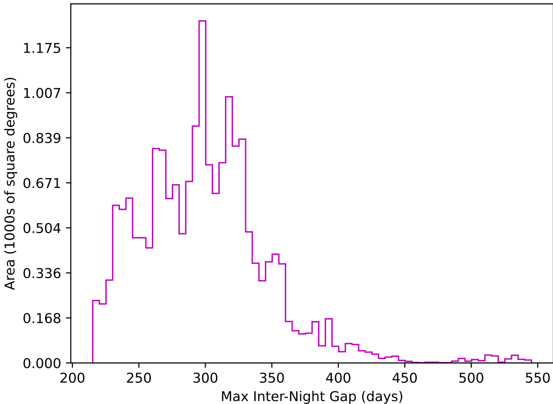
baseline_v3.5_10yrs WFD z band: Max Inter-Night Gap
