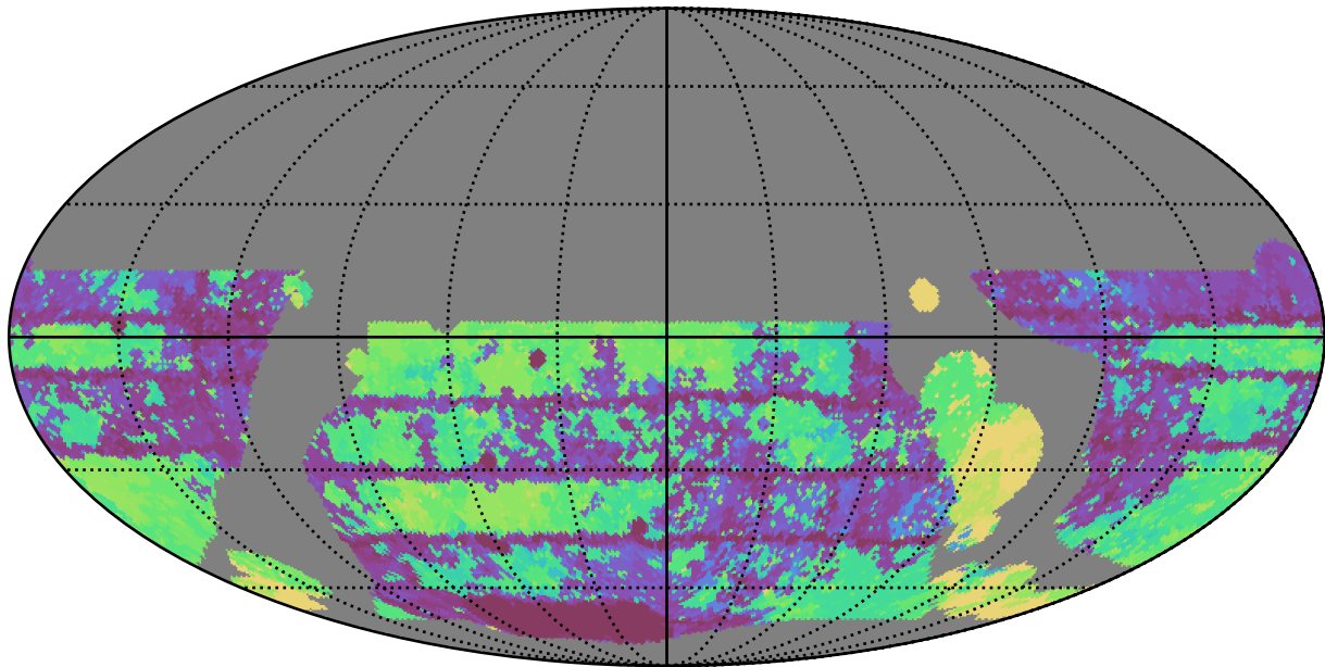
baseline_v3.5_10yrs WFD u band: Max Inter-Night Gap
