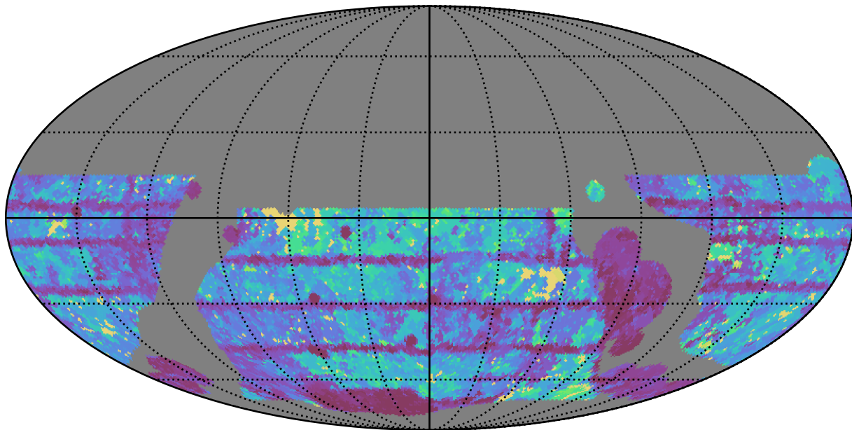
baseline_v3.5_10yrs WFD r band: Max Inter-Night Gap
