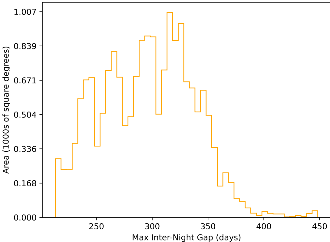
baseline_v3.5_10yrs WFD r band: Max Inter-Night Gap
