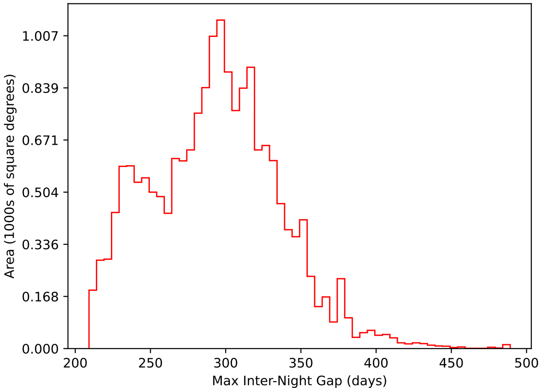
baseline_v3.5_10yrs WFD i band: Max Inter-Night Gap
