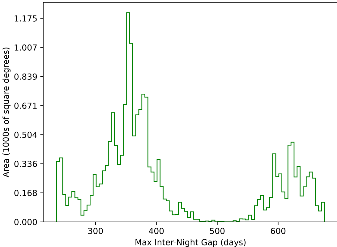
baseline_v3.5_10yrs WFD g band: Max Inter-Night Gap
