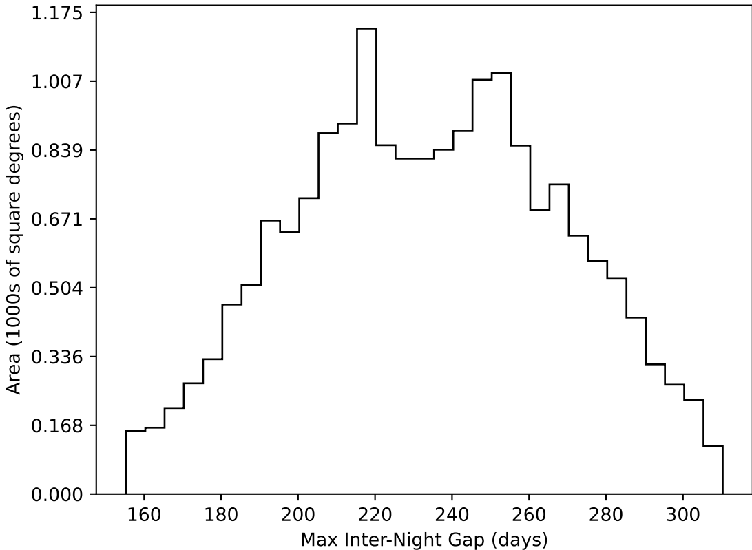
baseline_v3.5_10yrs WFD all bands: Max Inter-Night Gap
