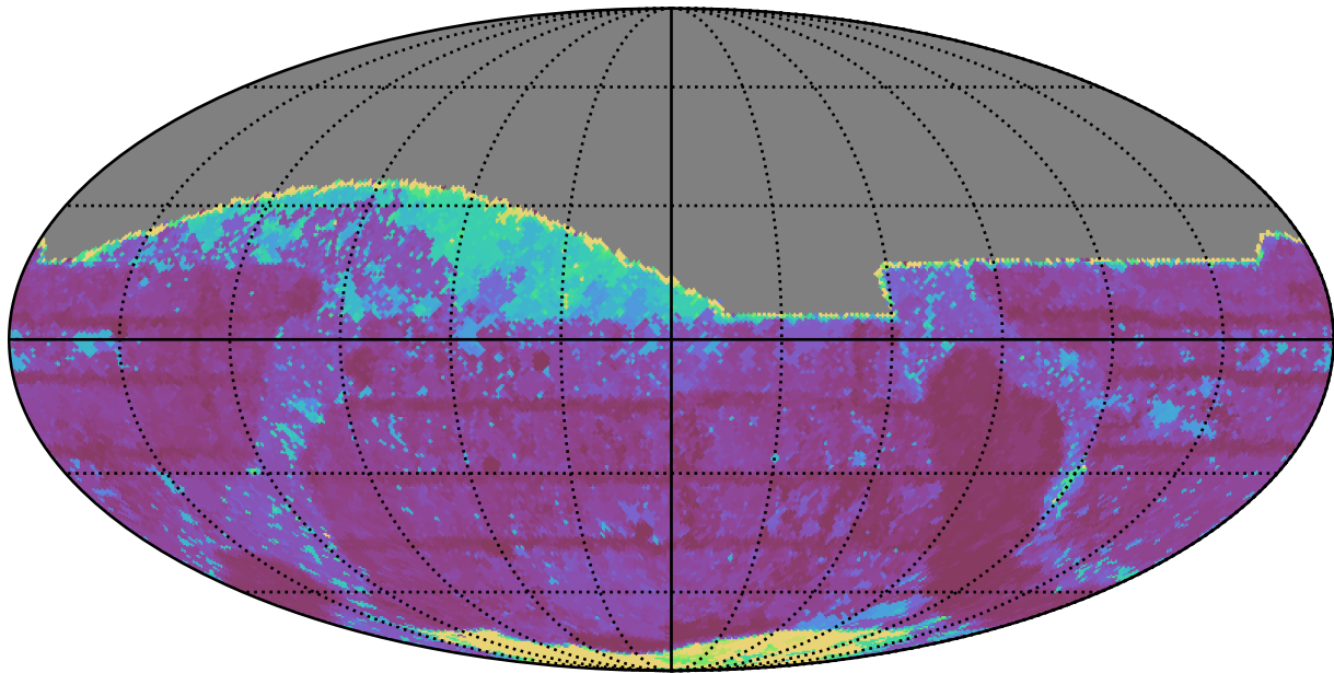
baseline_v3.5_10yrs All sky z band: Max Inter-Night Gap
