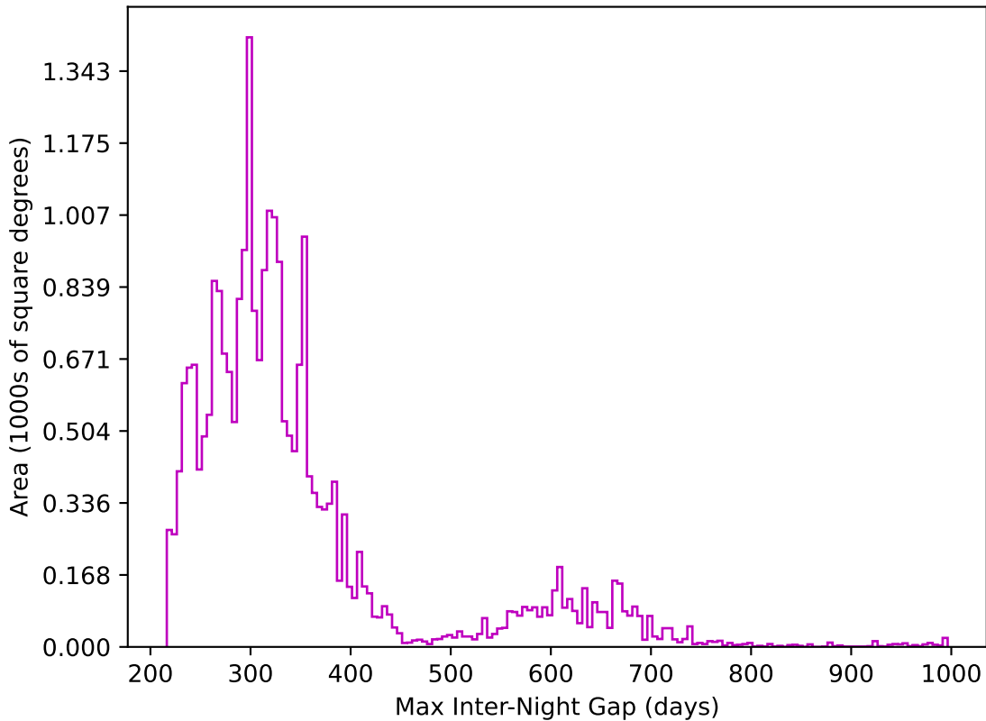
baseline_v3.5_10yrs All sky z band: Max Inter-Night Gap
