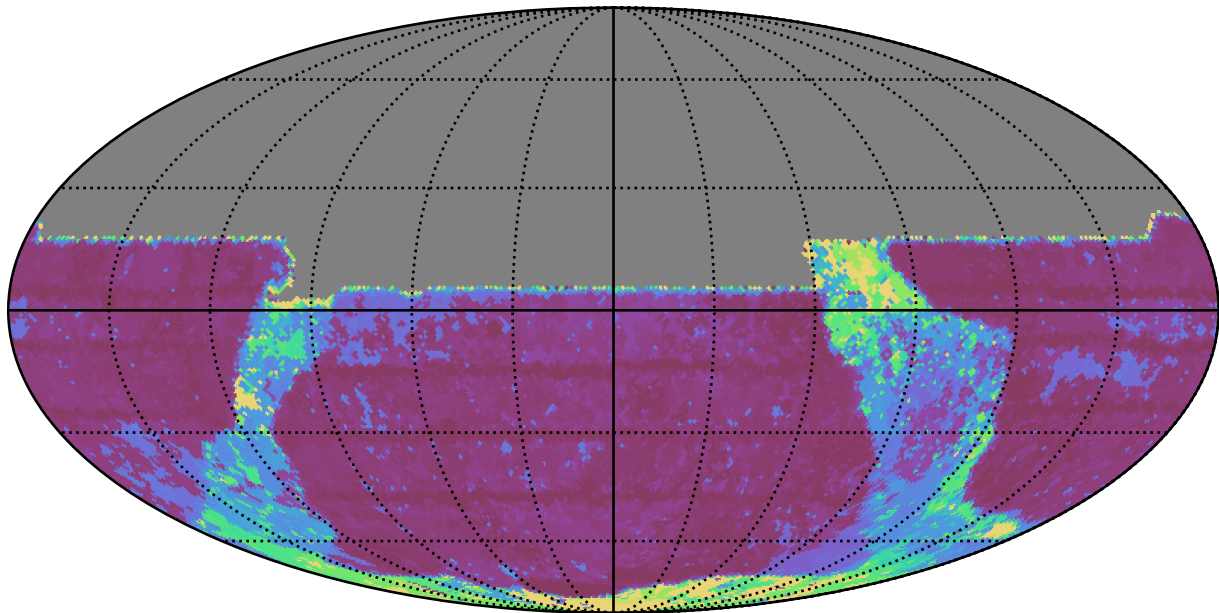
baseline_v3.5_10yrs All sky y band: Max Inter-Night Gap
