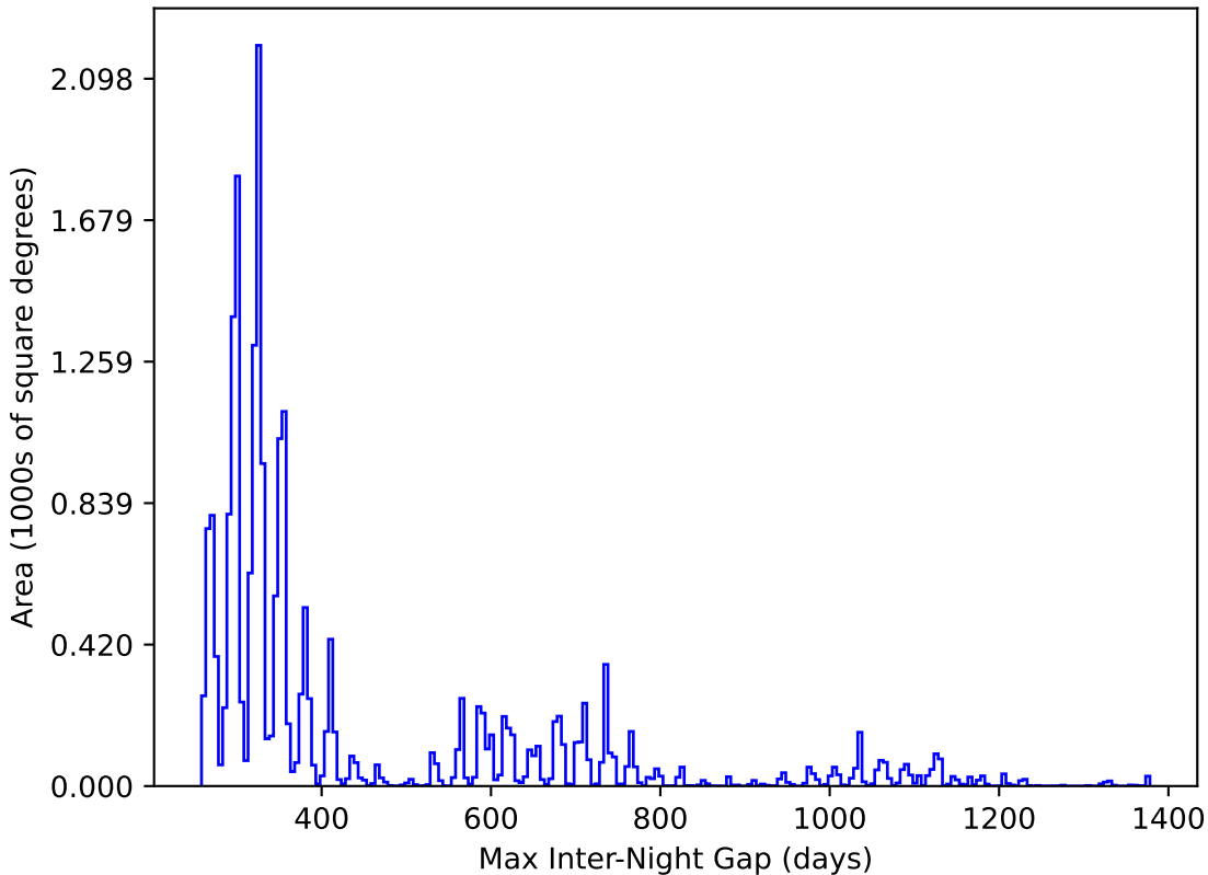
baseline_v3.5_10yrs All sky y band: Max Inter-Night Gap
