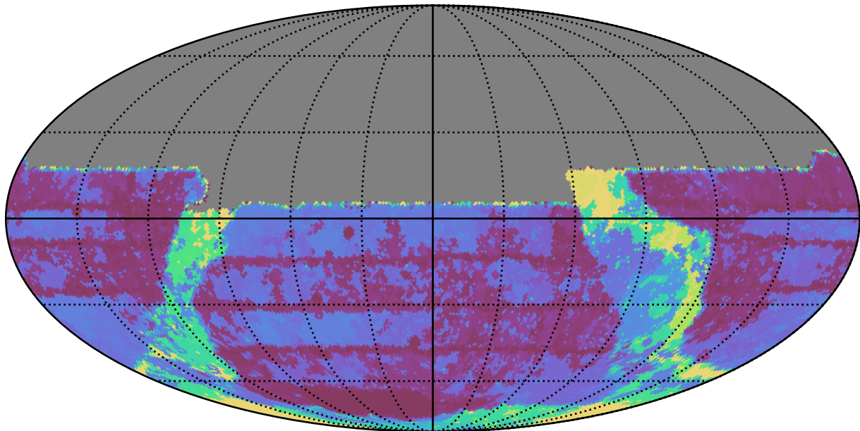
baseline_v3.5_10yrs All sky u band: Max Inter-Night Gap
