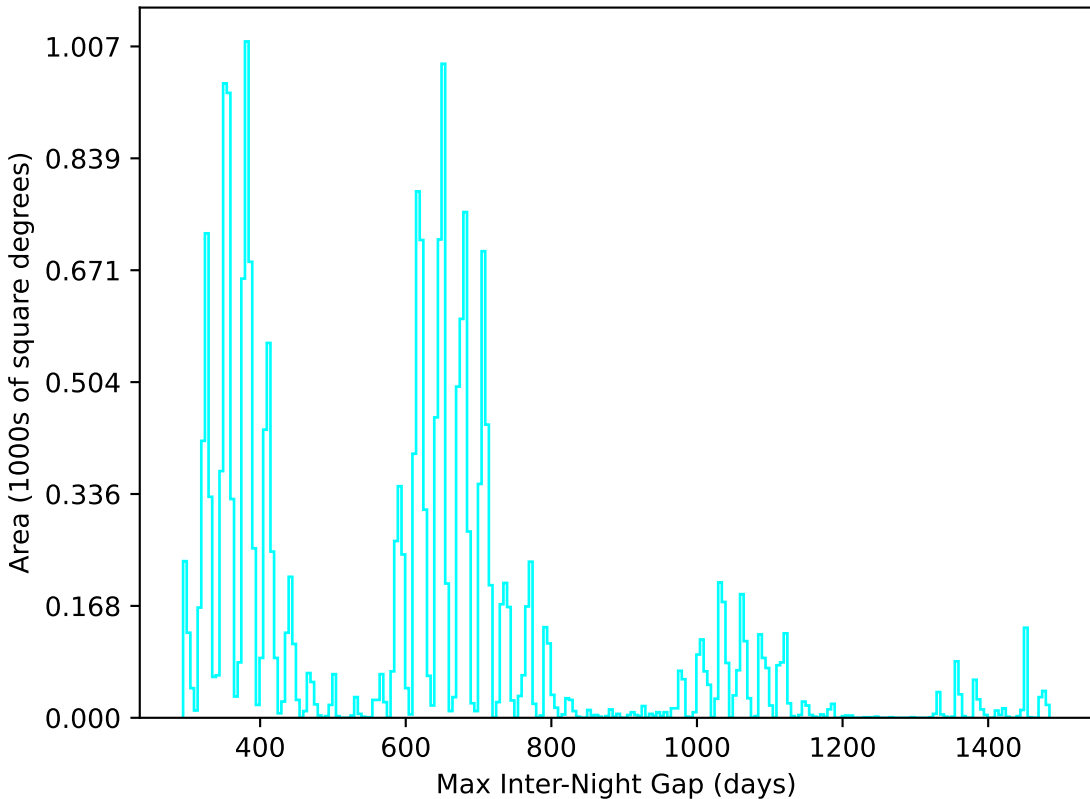
baseline_v3.5_10yrs All sky u band: Max Inter-Night Gap
