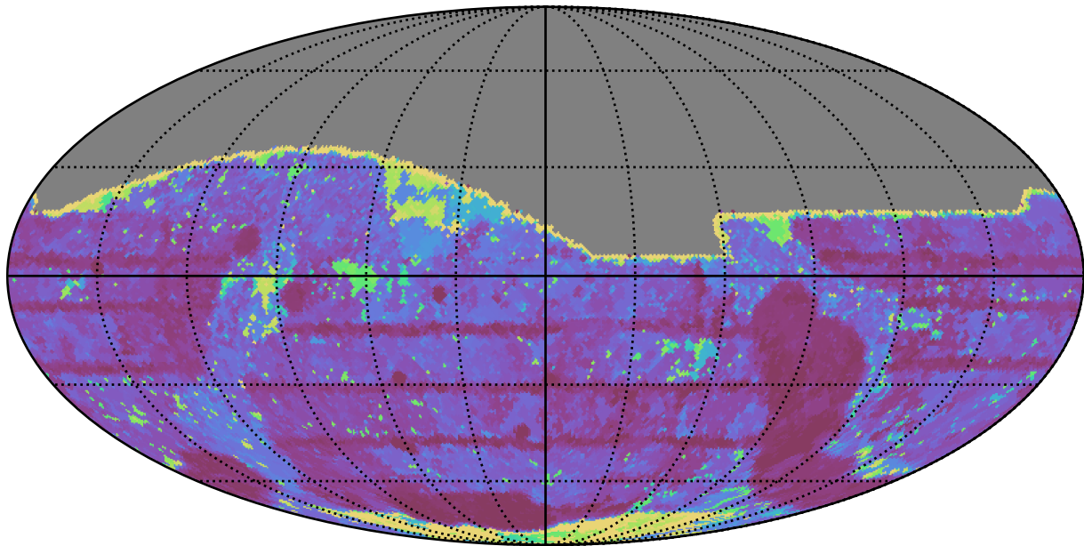
baseline_v3.5_10yrs All sky r band: Max Inter-Night Gap
