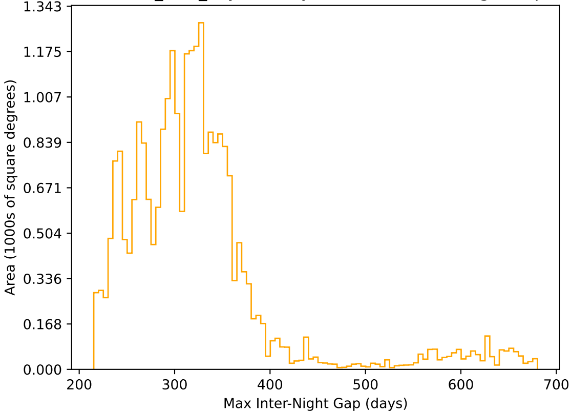
baseline_v3.5_10yrs All sky r band: Max Inter-Night Gap
