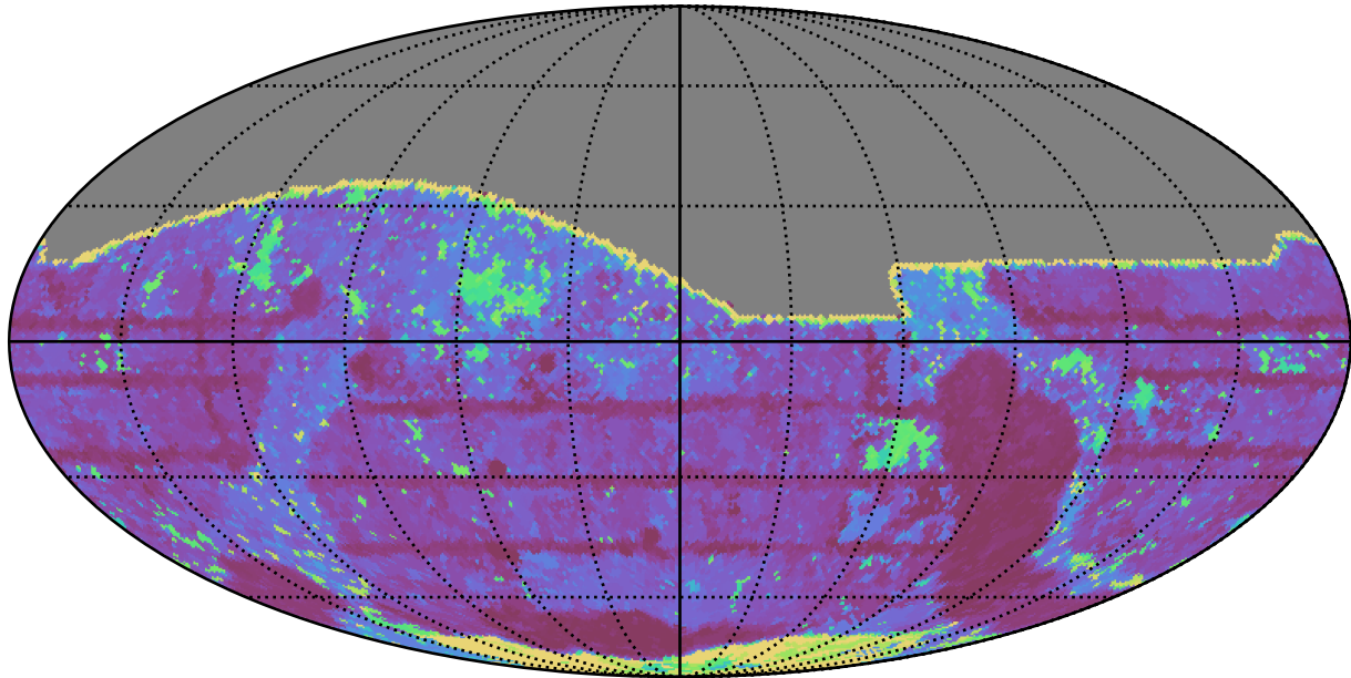
baseline_v3.5_10yrs All sky i band: Max Inter-Night Gap
