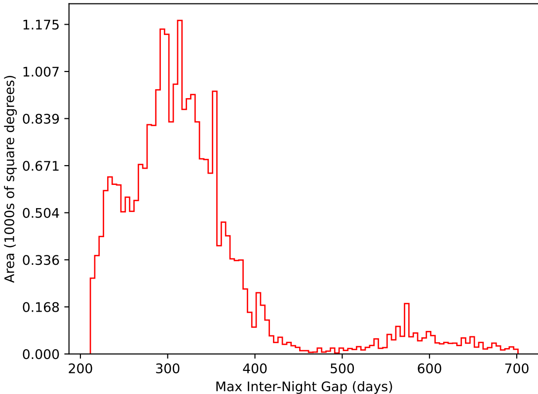
baseline_v3.5_10yrs All sky i band: Max Inter-Night Gap
