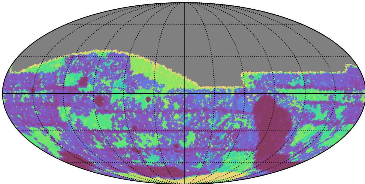
baseline_v3.5_10yrs All sky g band: Max Inter-Night Gap
