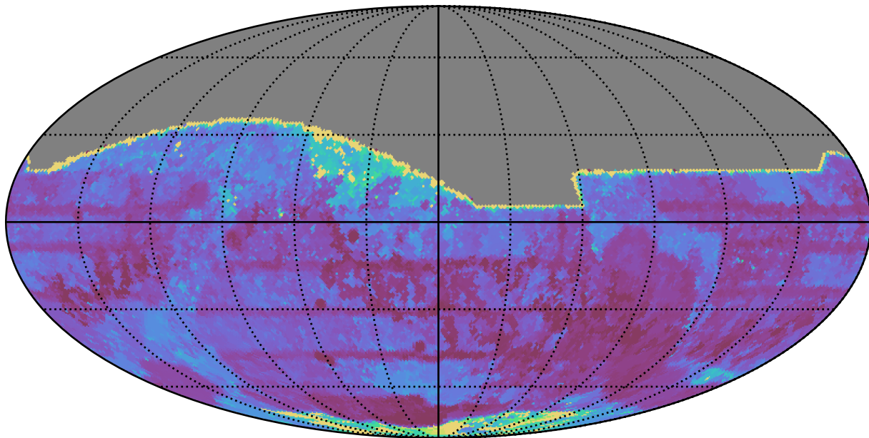
baseline_v3.5_10yrs All sky all bands: Max Inter-Night Gap
