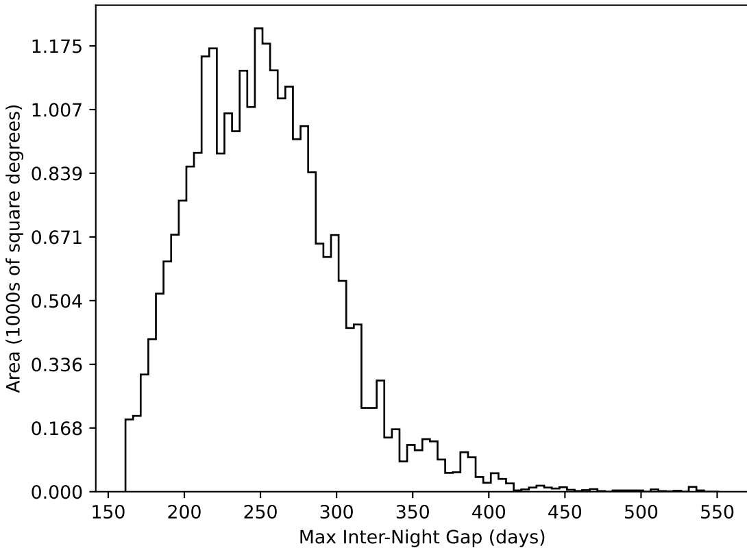
baseline_v3.5_10yrs All sky all bands: Max Inter-Night Gap
