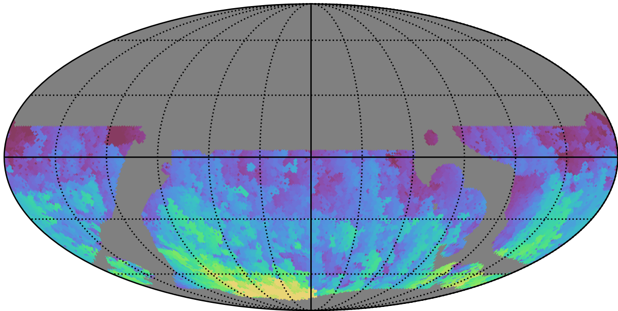
baseline_v3.5_10yrs WFD u band: Max HA
