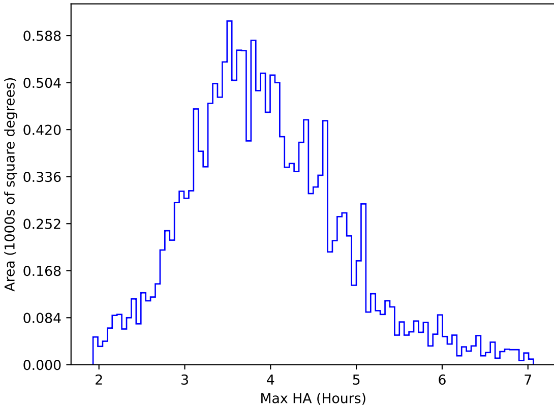
baseline_v3.5_10yrs WFD u band: Max HA
