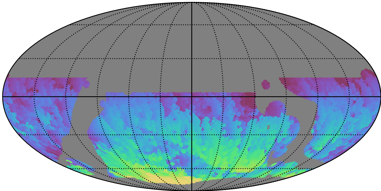
baseline_v3.5_10yrs WFD r band: Max HA
