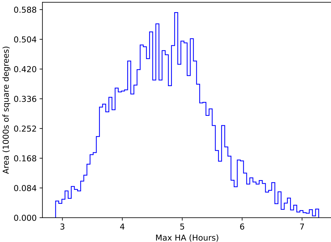
baseline_v3.5_10yrs WFD r band: Max HA
