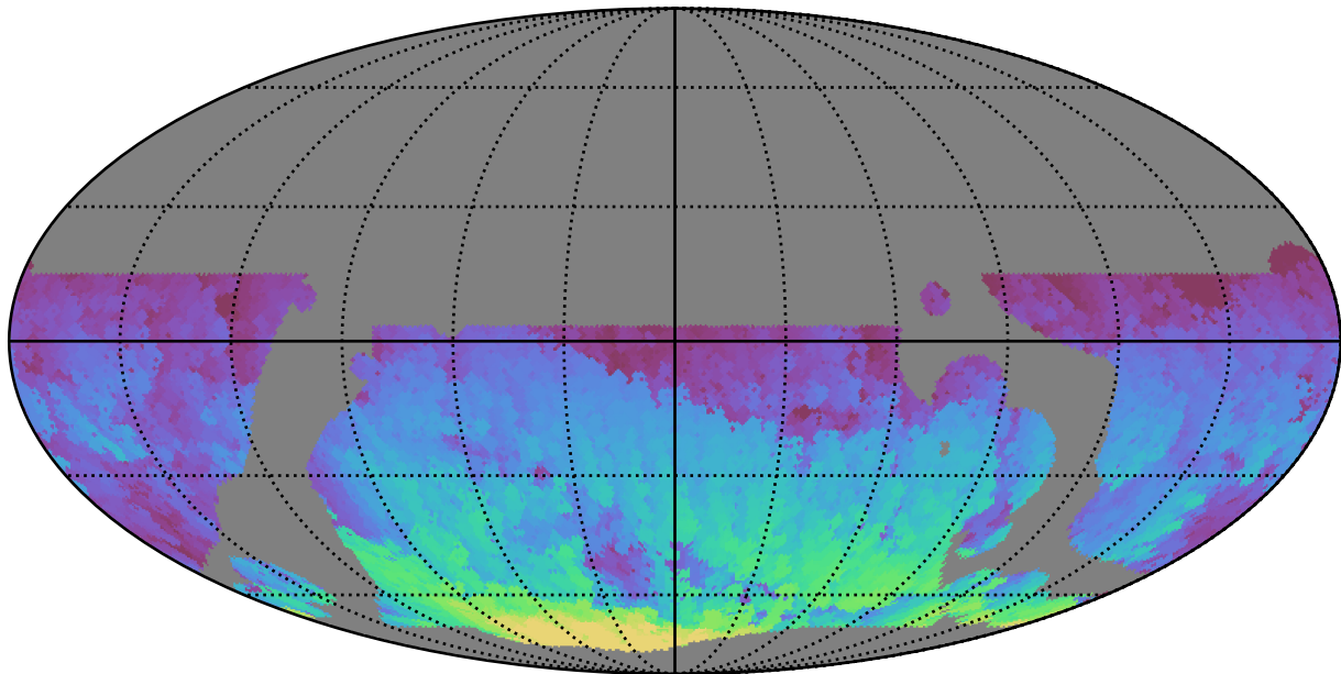
baseline_v3.5_10yrs WFD i band: Max HA
