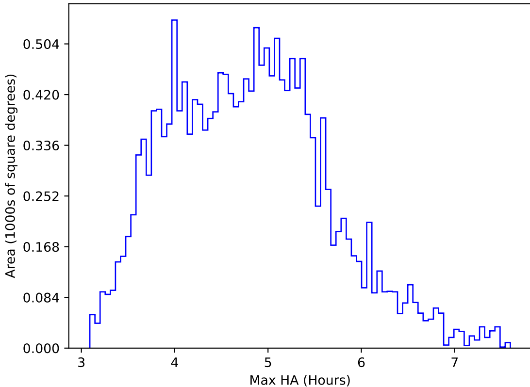
baseline_v3.5_10yrs WFD i band: Max HA
