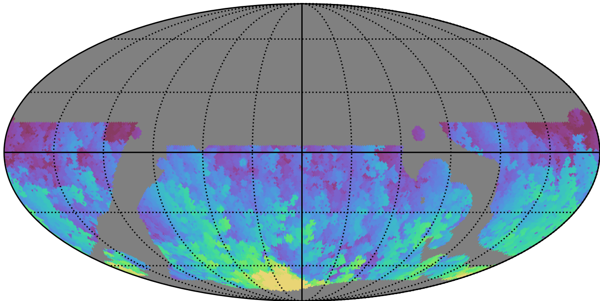
baseline_v3.5_10yrs WFD g band: Max HA
