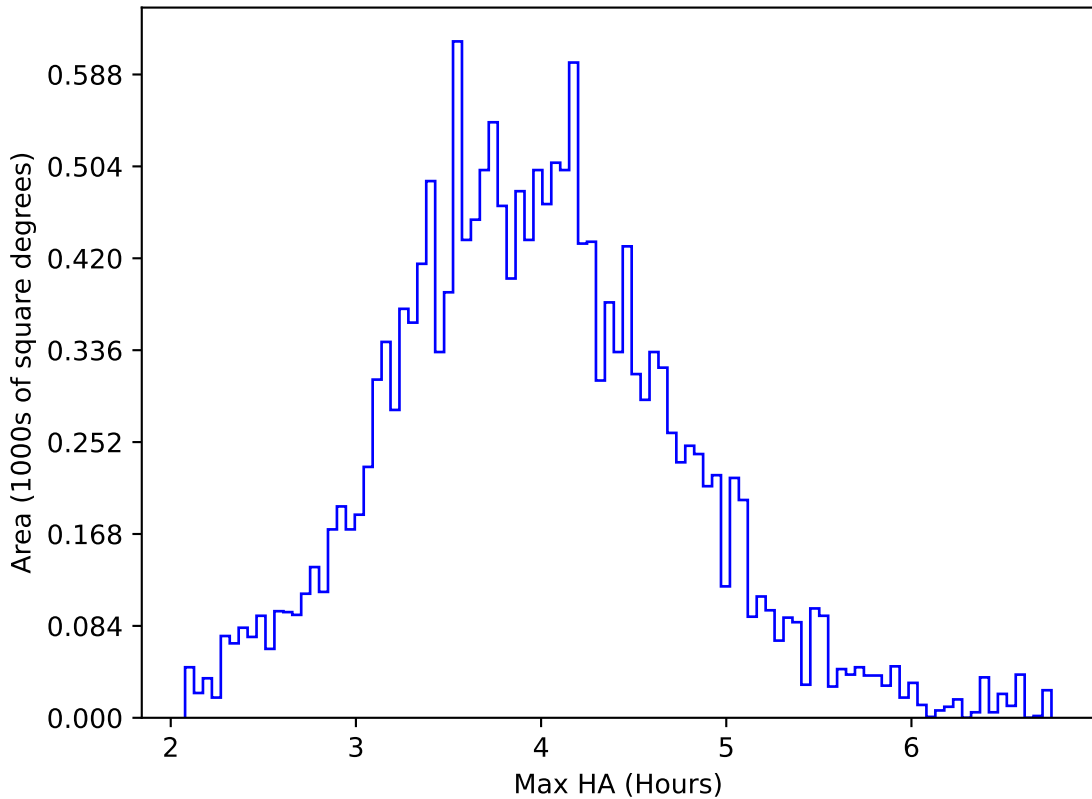
baseline_v3.5_10yrs WFD g band: Max HA
