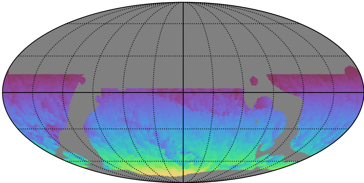
baseline_v3.5_10yrs WFD all bands: Max HA
