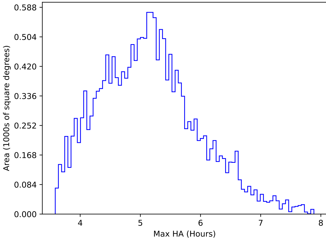
baseline_v3.5_10yrs WFD all bands: Max HA
