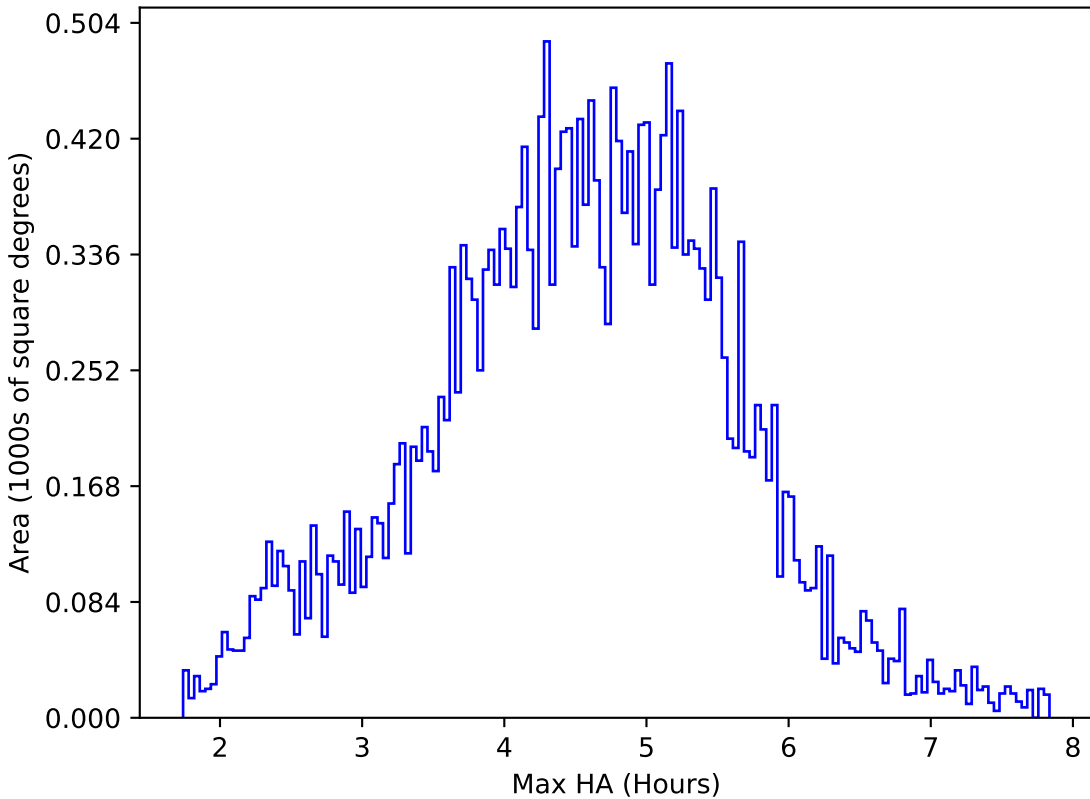
baseline_v3.5_10yrs All sky z band: Max HA
