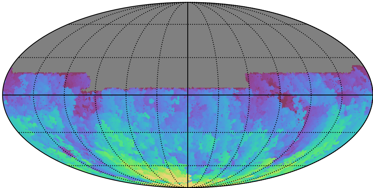
baseline_v3.5_10yrs All sky u band: Max HA
