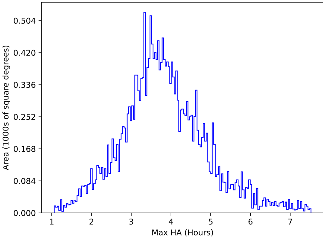
baseline_v3.5_10yrs All sky u band: Max HA
