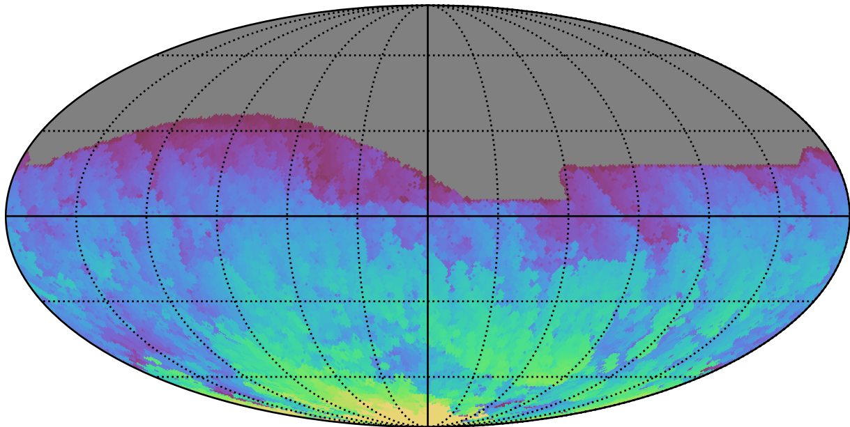
baseline_v3.5_10yrs All sky r band: Max HA
