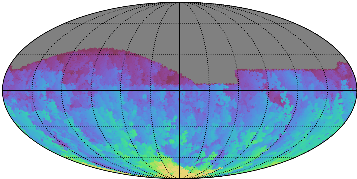
baseline_v3.5_10yrs All sky g band: Max HA
