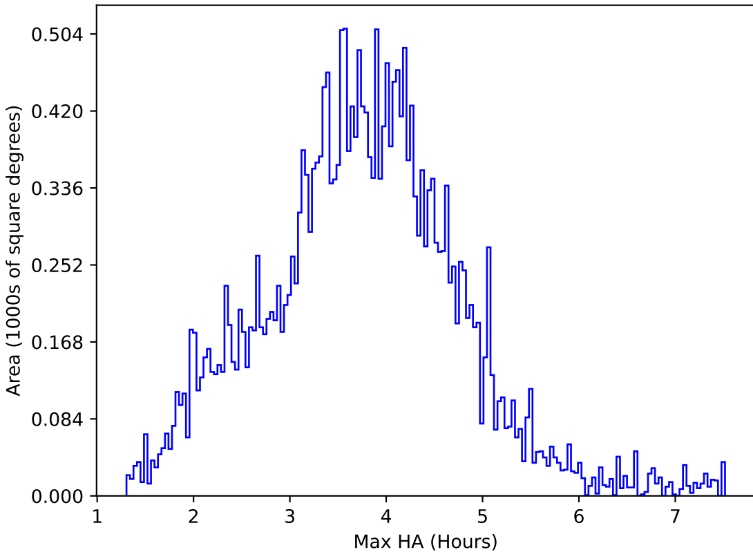
baseline_v3.5_10yrs All sky g band: Max HA
