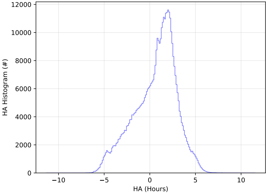
baseline_v3.5_10yrs WFD z band: HA Histogram
