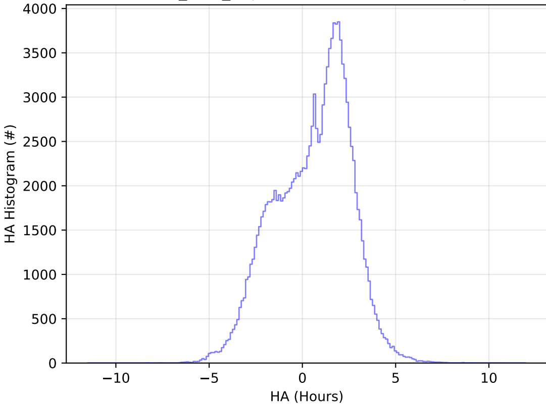
baseline_v3.5_10yrs WFD u band: HA Histogram
