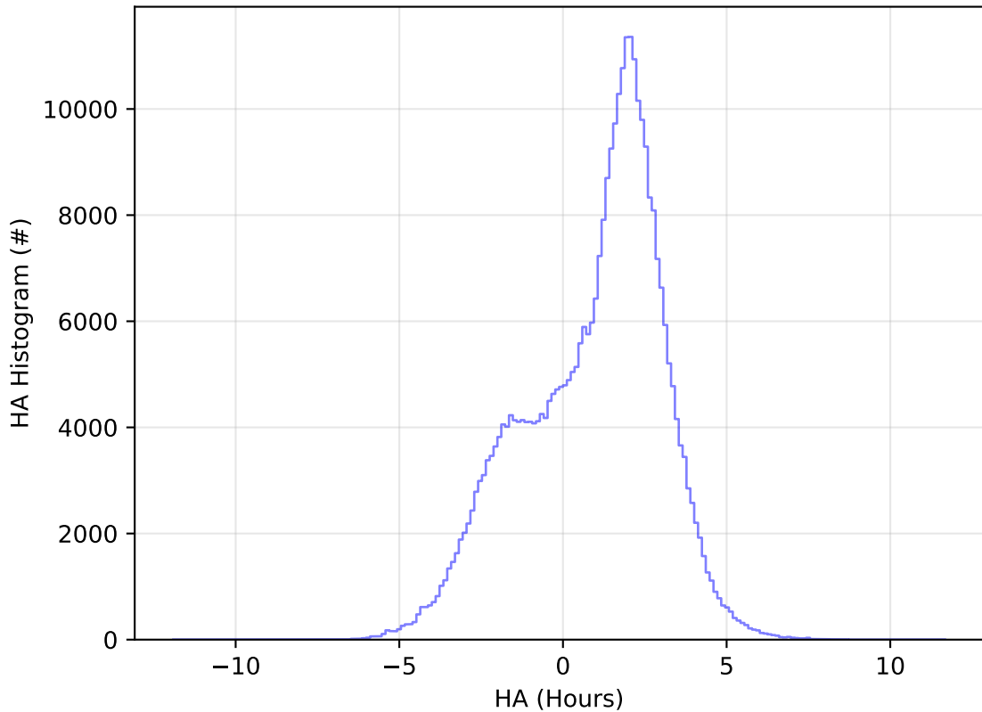
baseline_v3.5_10yrs All sky y band: HA Histogram
