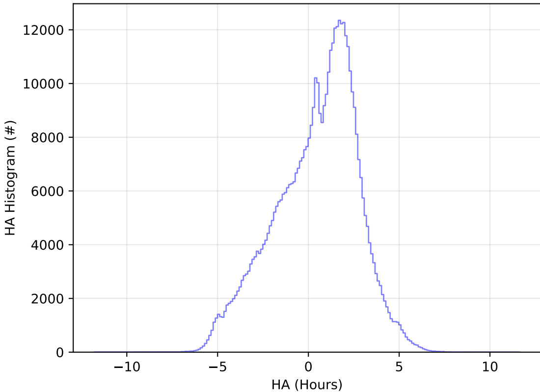
baseline_v3.5_10yrs All sky r band: HA Histogram
